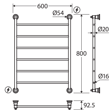
⚡ Wiring Positions
