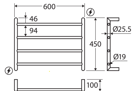
⚡ Wiring Positions
