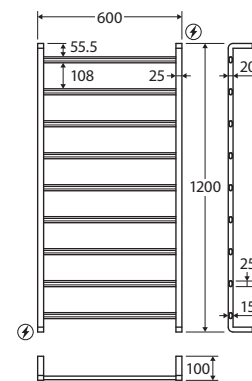
⚡ Wiring Positions
