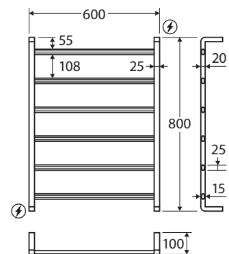
⚡ Wiring Positions
